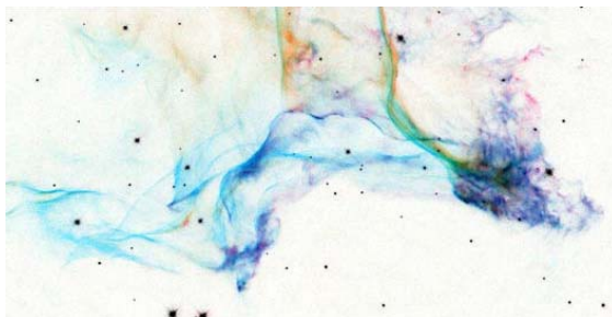
Supernova remnant (negative image)
